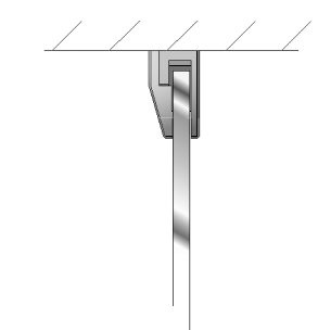
5 Connection of partition wall to brick wall
